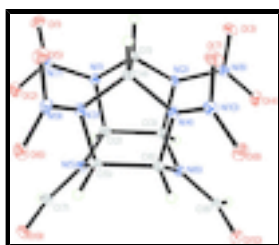
Fig. 1. The structure of PTNDFIW, with displacement ellipsoids drawn at the 50% probability level.
